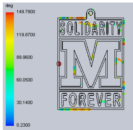
Figure 14. Simulation result at 240°C optimal injection condition
