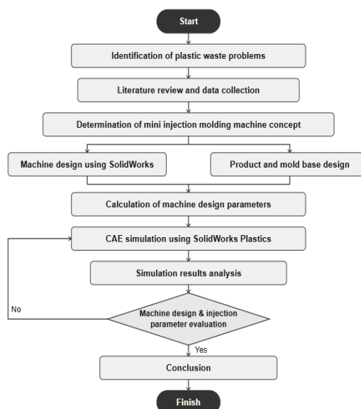
Figure 1. Research Flowchart
