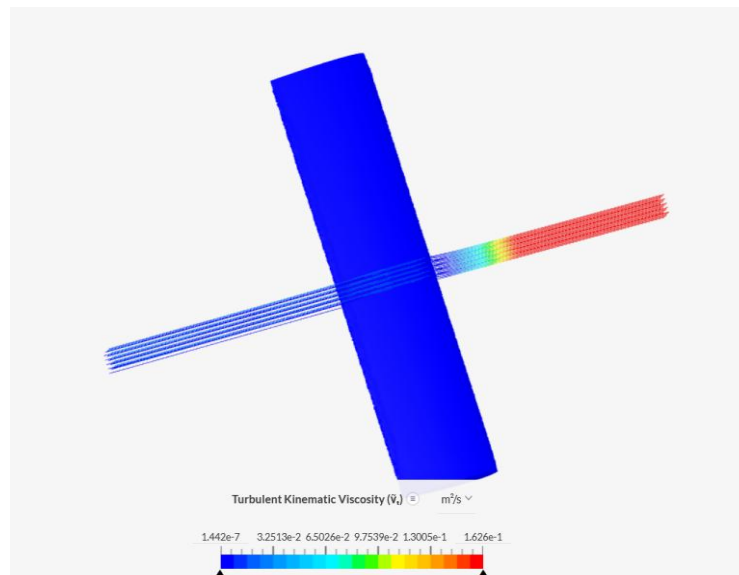
Figure 14. Distribution of v_t NACA 0012 angle of attack 5^\circ
