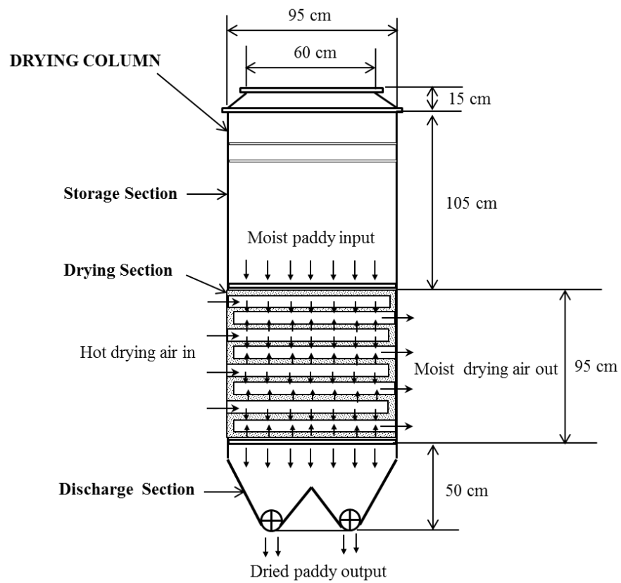
Figure 3. Schematic of the drying column with dimensions.
