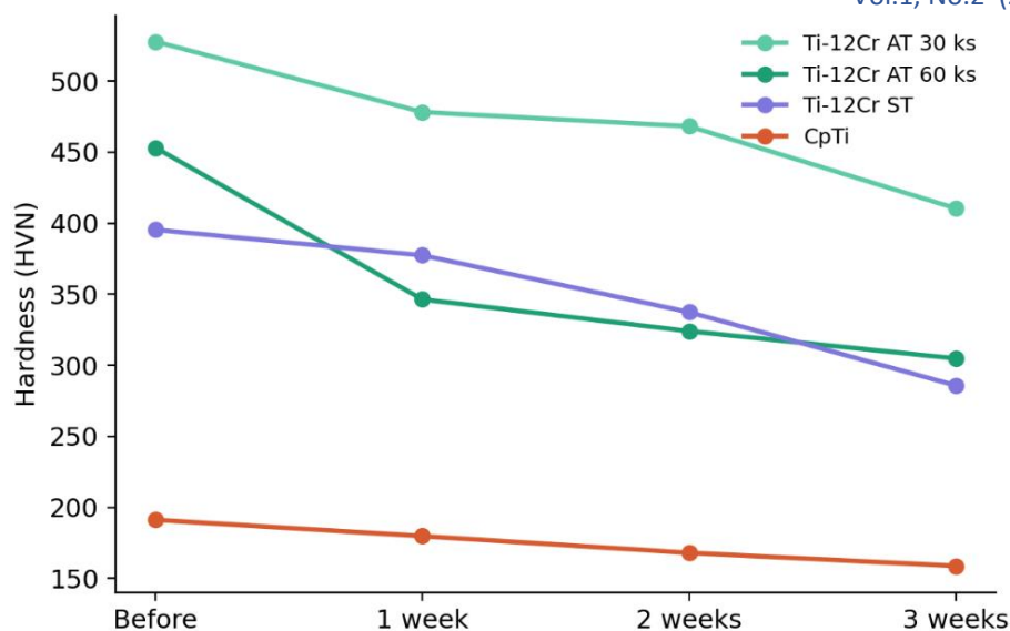
Figure 8. Hardness values of the four material conditions with respect to immersion time.
