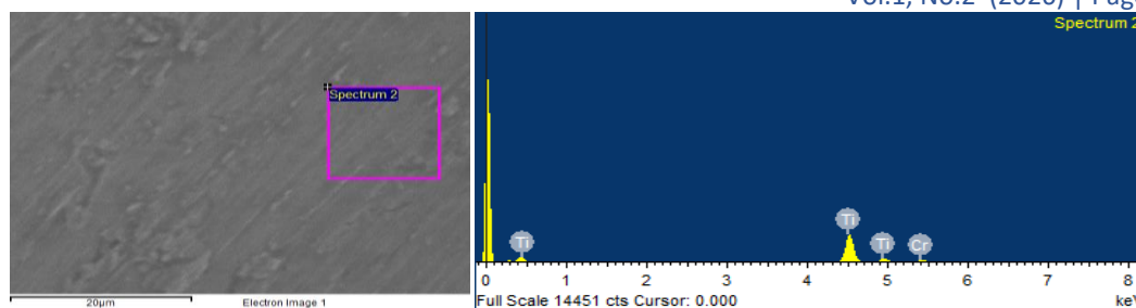
(b) Ti-12Cr AT 30 ks
