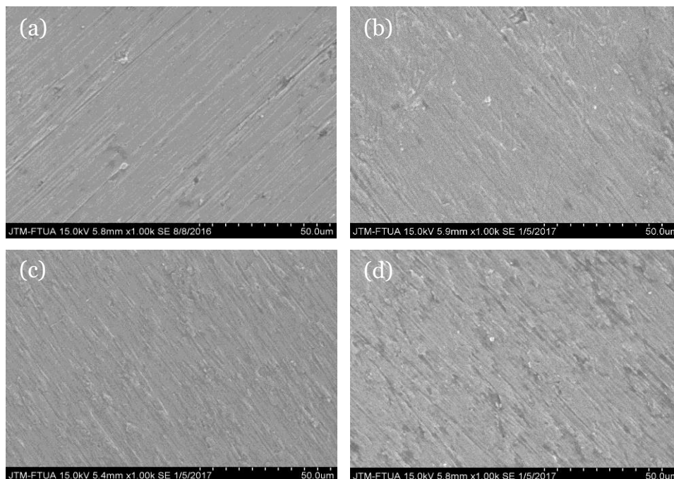
Figure 7. Surface morphology of CpTi under the conditions of (a) before testing, (b) 1 week, (c) 2 weeks, and (d) 3 weeks of immersion.
