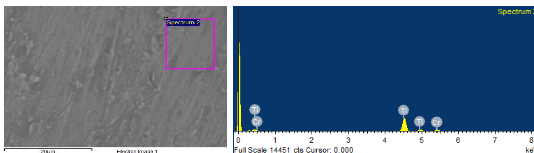
(c) Ti-12Cr AT 60 ks
