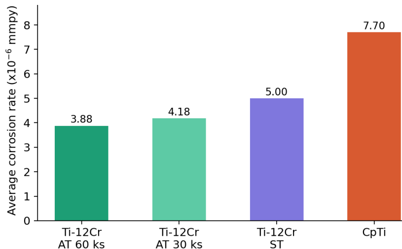
Figure 5. Comparison of the average corrosion rates of the four material conditions.
