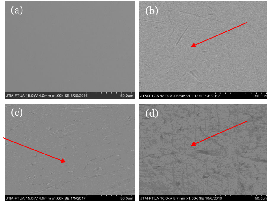
Figure 6. Surface morphology of Ti-12Cr AT 60 ks under the conditions of (a) before testing, (b) 1 week, (c) 2 weeks, and (d) 3 weeks of immersion.
