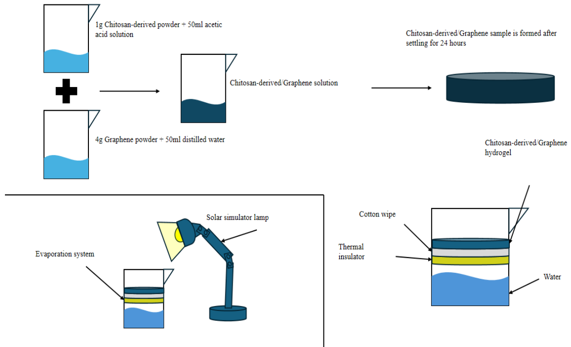
Figure 2. Fabrication process for producing chitosan-derived/graphene hydrogel.
