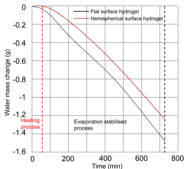
Figure 9. Water mass changes of the flat-surface hydrogel and the hemispherical-surface hydrogel samples under solar simulator irradiation for up to 12 hours.
