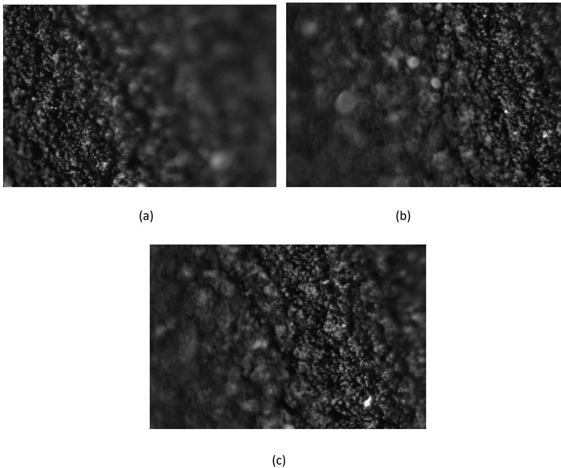
Figure 7. Surface morphology of the hemispherical-surface hydrogel sample.
