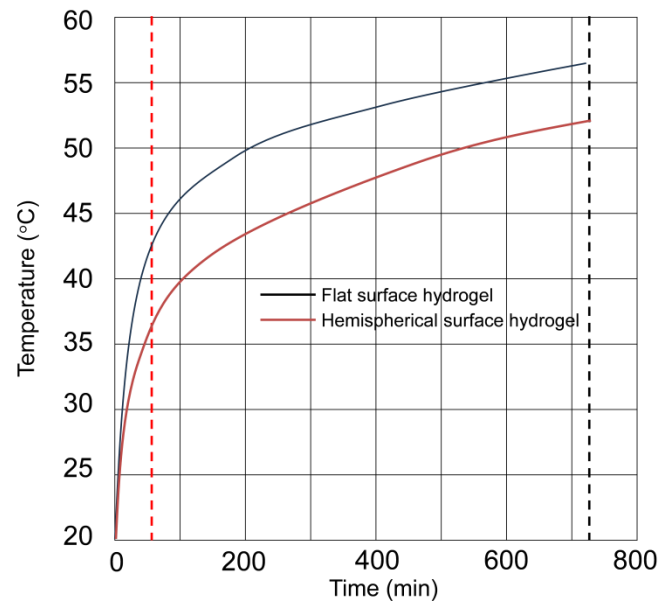
Figure 8. Temperature distribution of the flat-surface hydrogel and hemispherical-surface hydrogel samples under solar simulator irradiation for up to 12 hours.
